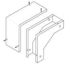
90 DEG VERTICAL OUTSIDE RISER
