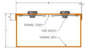
SPECIAL QUICK-RELEASE TURNBUCKLE TYPE COVER TRUNKING
