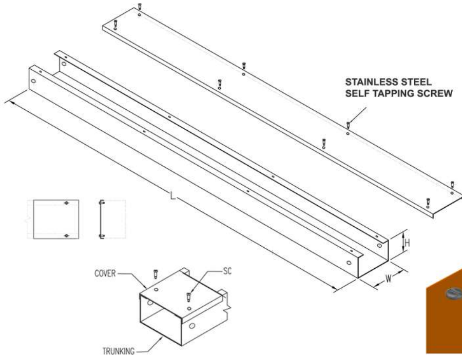
STANDARD SELF TAPPING SCREW COVER TRUNKING
