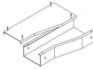
RIGHT HAND REDUCER
