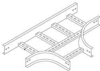
90 DEG HORIZONTAL EQUAL TEE
