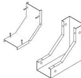
90 DEG VERTICAL INSIDE RISER
