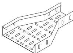
OFFSET STRAIGHT REDUCER
