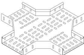
90 DEG HORIZONTAL EQUAL CROSS
